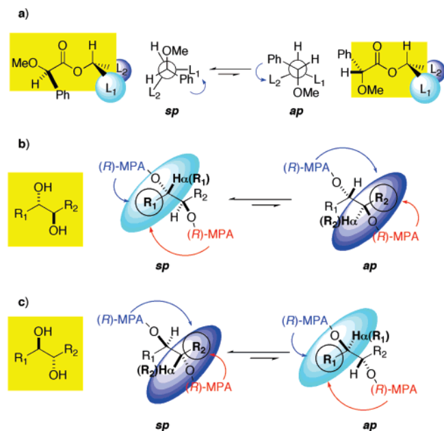
FIGURE 4. (a) Structure and equilibrium between the sp and ap conformers of the (R) -MPA ester of a secondary alcohol. (b and c) Distribution of the shielding effects for the bis- (R) -MPA esters of anti C and anti D diols, respectively.
