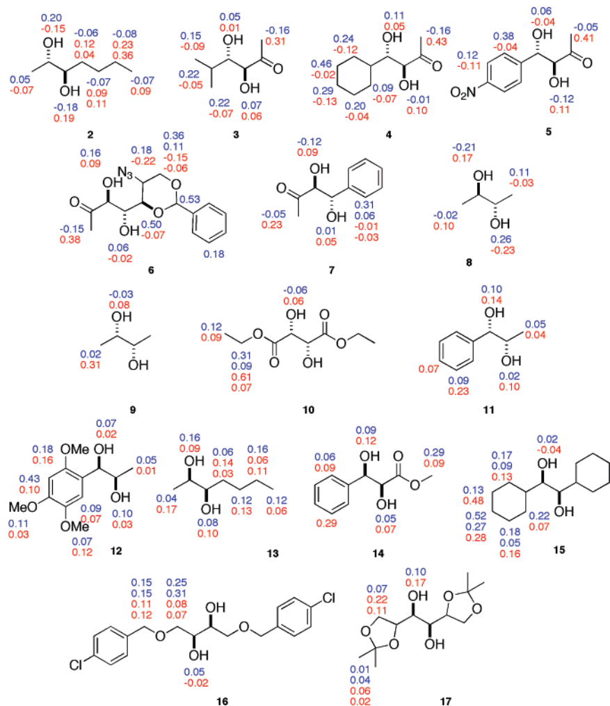
FIGURE 3. Selection of 1,2-secondary/secondary diols employed in this study, and \Delta\delta^{T1T2} values (ppm, 298–183 K, CS_2/CD_2Cl_2 , 4:1) obtained for their bis-( R )-MPA (blue) and bis-( S )-MPA esters (red).
