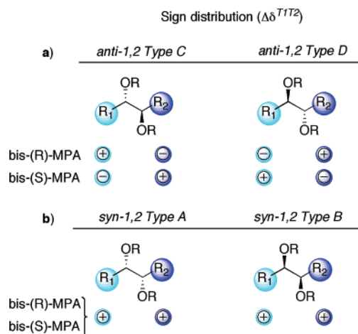
FIGURE 6. \Delta\delta^{T1T2} sign distributions for the bis- (R) - and (S) -MPA esters of anti (a) and syn (b) 1,2-secondary/secondary diols
